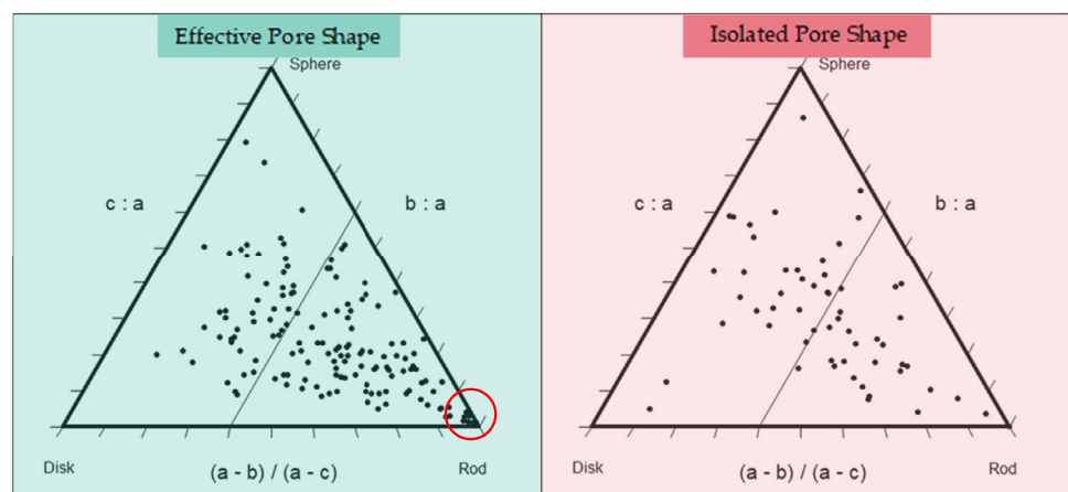
Fig. 5 Pore space shape distribution in natural flocs, divided into hydraulically effective and isolated pore spaces. Circle in effective pore shape plot indicates a zone where a large portion of the n is situated
