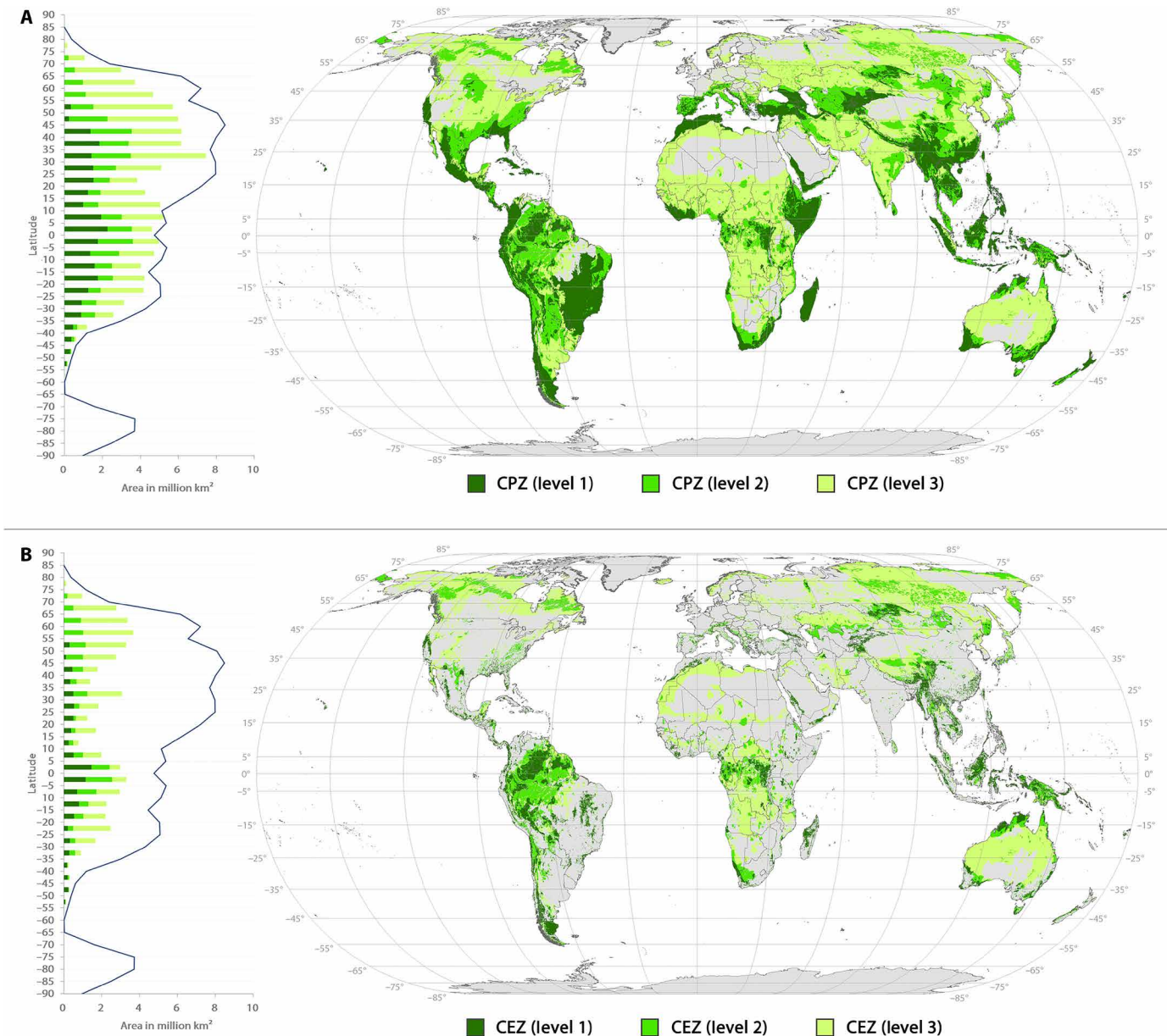
Fig. 1. Global distribution of CPZs and CEZs. (A) distribution of CPZs. (B) distribution of CEZs. Charts on the left show the latitudinal distribution of CPZs and CEZs, in which polylines represent the total land area at the corresponding latitude.
